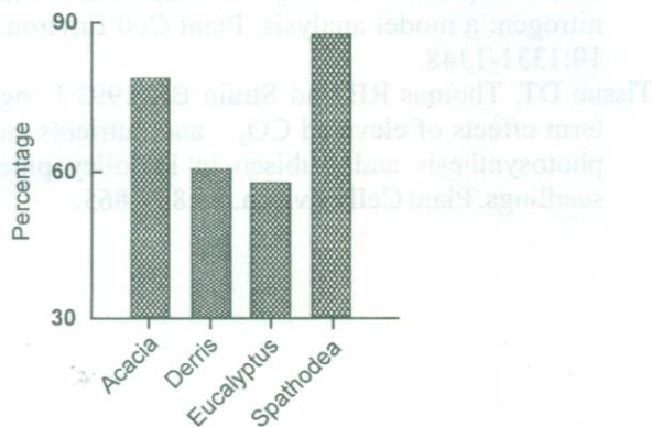
Fig. 2. Percent increase in photosynthesis when measured at elevated \text{CO}_2 concentration of 660 \mu\text{mol mol}^{-1} in four different tree seedlings.
