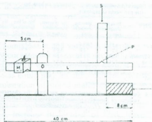
Fig.1 : Husk compression measurement device M- Compression load (= 645.0g), L- Lever, P- Pointer, E-Support, S-Graduated scale
