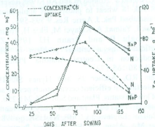
Fig. 2. Influence of N and P application on Zn concentration and crop uptake at different stages of growth in wheat.
